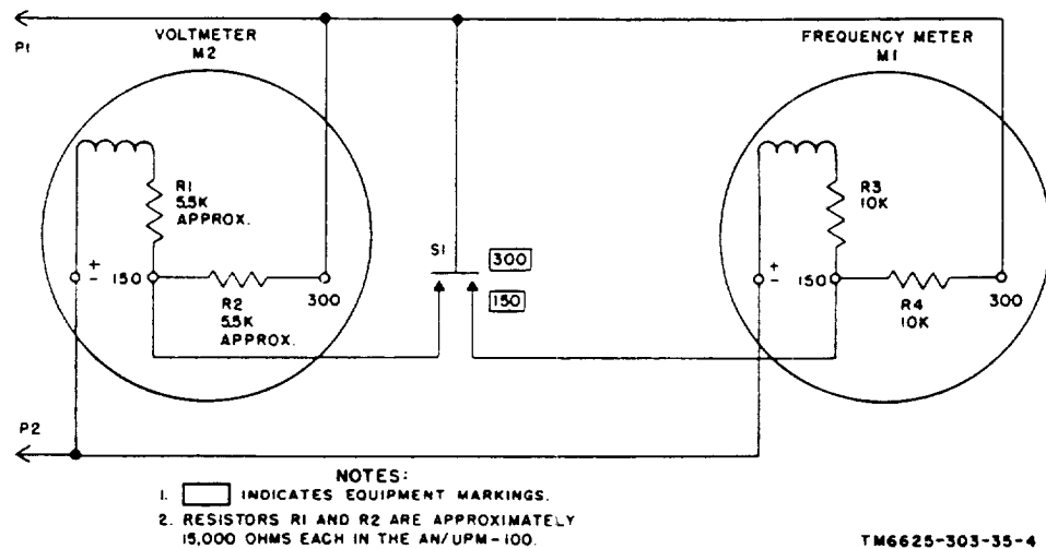
Figure 1. Schematic diagram.
